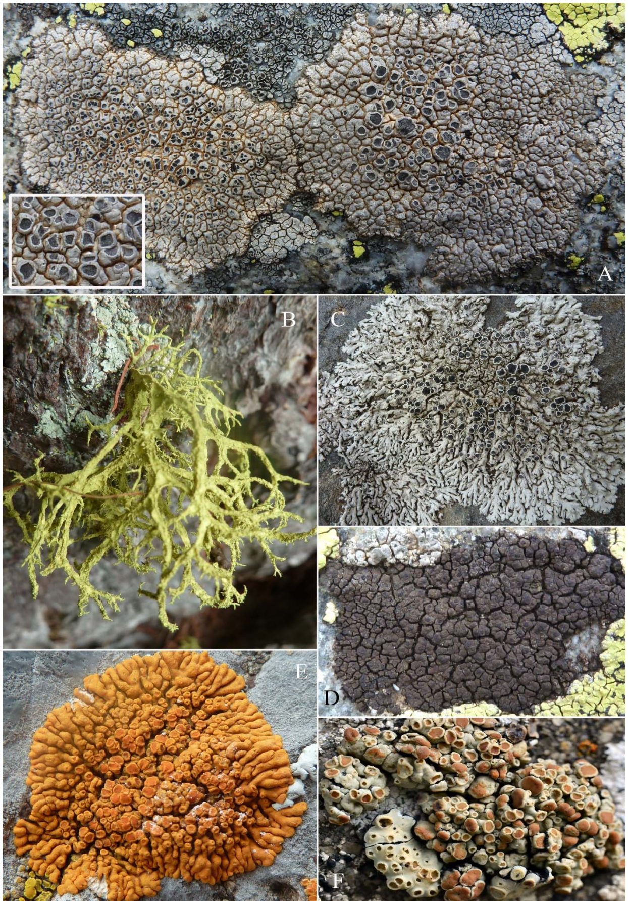
J1b. A. Aspicilia polychroma subsp. polychroma (JPG). B. Letharia vulpina (MCD). C. Physcia albinea (JPG). D. Staurothele areolata . (JPG). E. Caloplaca biatorina . F. Rhizoplaca peltata (FJ).
